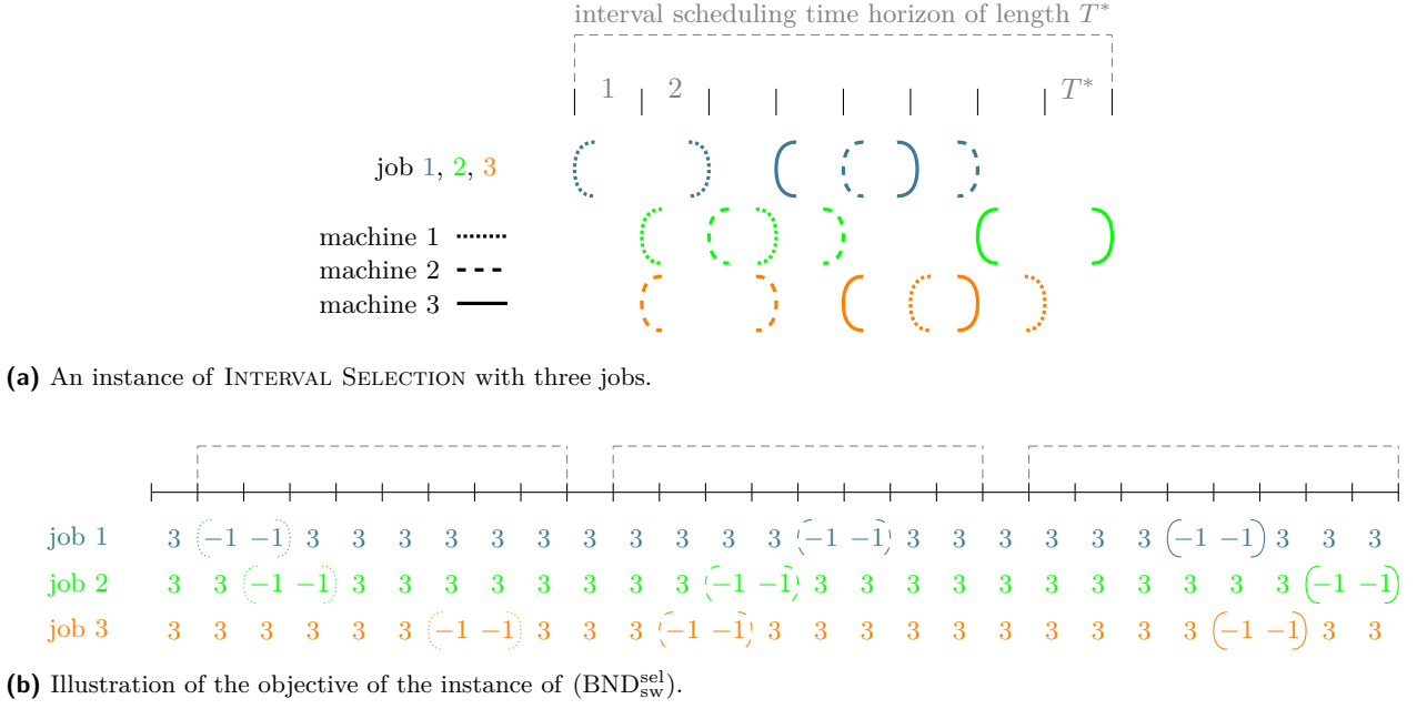
■ Figure 1 Illustration of the reduction in the proof of Theorem 7.
