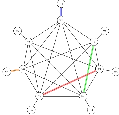
(b) Corresponding matching in G .
