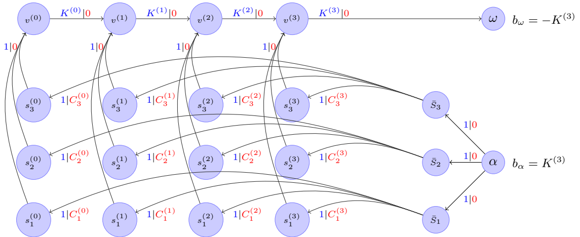
■ Figure 2 Sketch of the network constructed in the proof of Theorem 12, for n = 3 and T = 3 . All edges are labeled by capacity and cost, where C_i^{(t)} := \sum_{j=t}^T c_i^{(j)} for all t \in \{0, 1, 2, 3\} .
